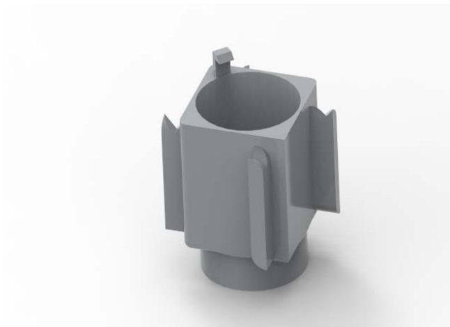
Figure 3. A rendered picture of the engine mount with 4 vortex generators
