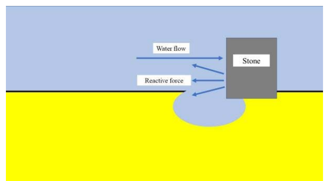
Figure 2 Detailed process
